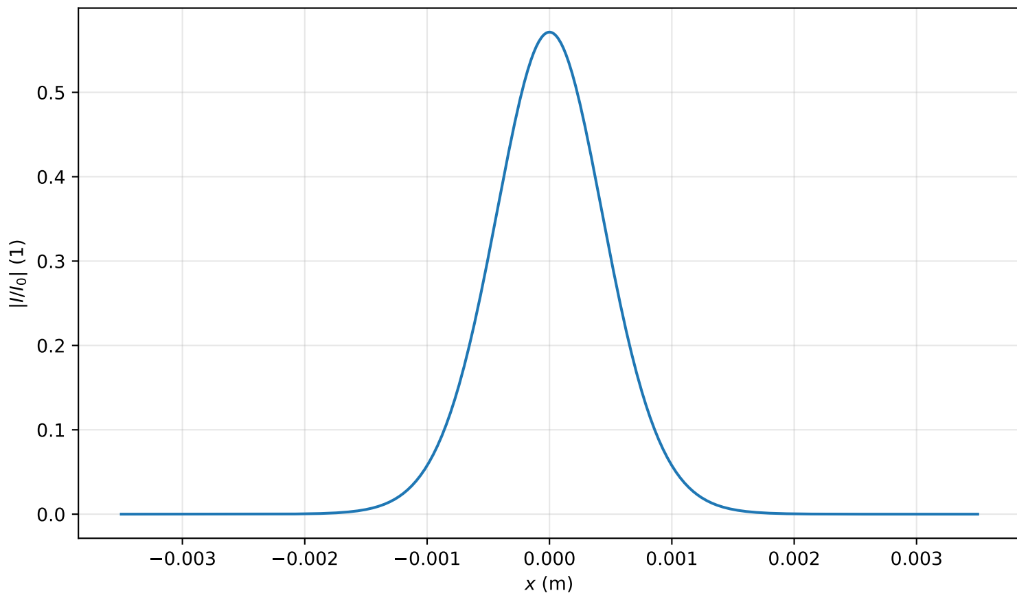
Intensity profile I(x, y = 0, z = 2.309m)/I_0 , P_{in}=0.3P_{cr} , artificial time
